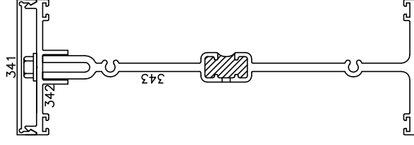
3-PIECE MULLION
