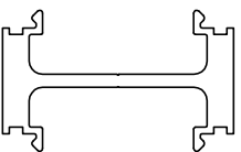
STRUCTURAL MULLION HORIZONTAL OR VERTICAL
