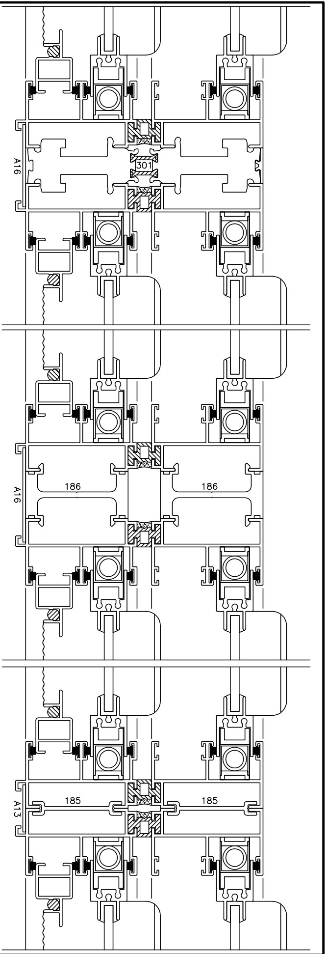
IMPACT MULLION HORIZONTAL OR VERTICAL
