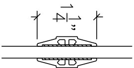
PROFILE APPLIED MUNTIN (BOTH SIDES) SCW-223
