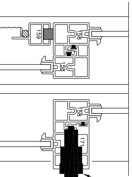
920 DOUBLE HUNG WITH OPTIONAL KEY LOCK
