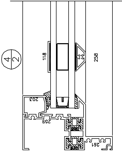
TYPICAL UPPER JAMB DETAIL (4/2)
